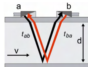
Transit time measurement technology as applied by Katronic's flowmeters.
